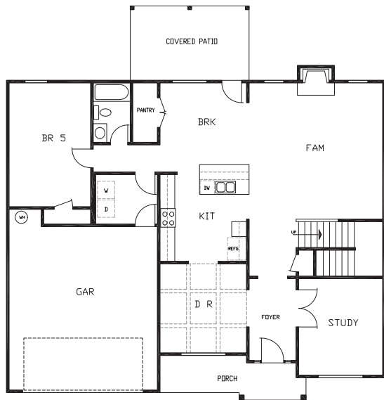
1ST FLOOR
