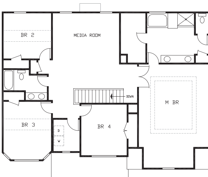
2ND FLOOR
