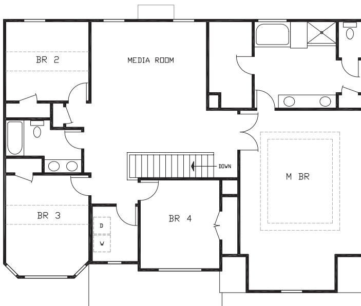
2ND FLOOR
