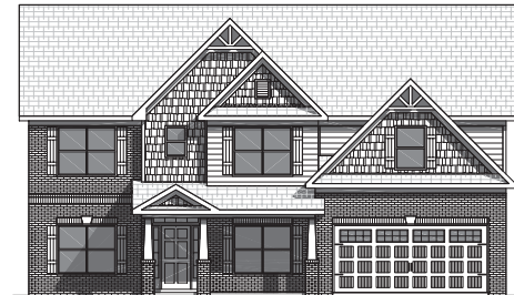
ELEVATION D
