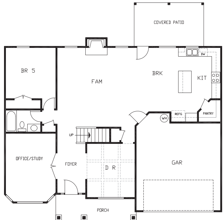
1ST FLOOR
