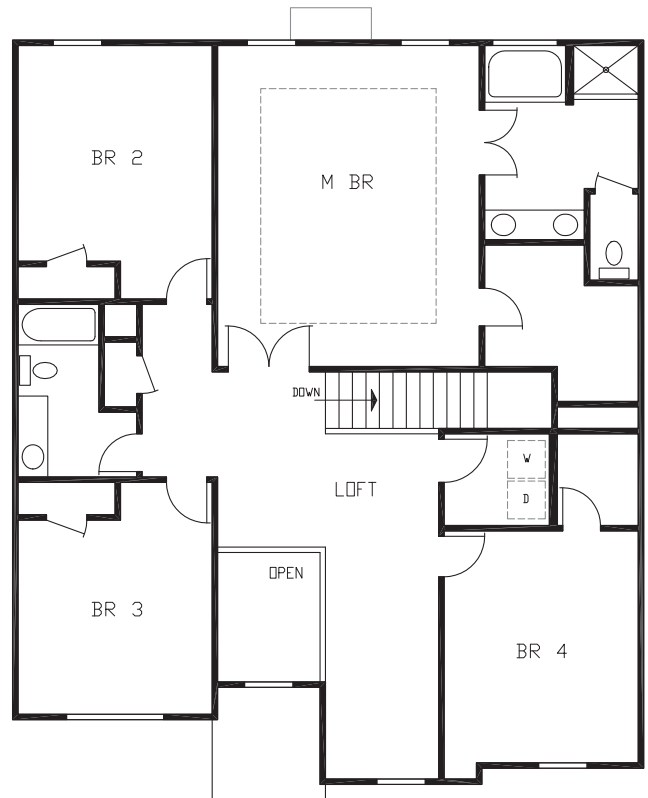
2ND FLOOR
