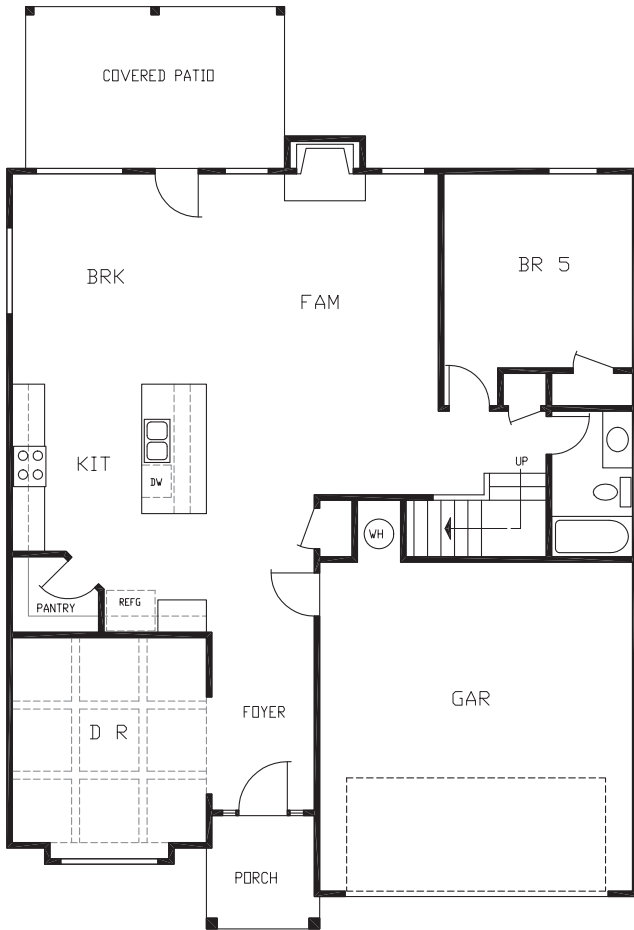
1ST FLOOR
