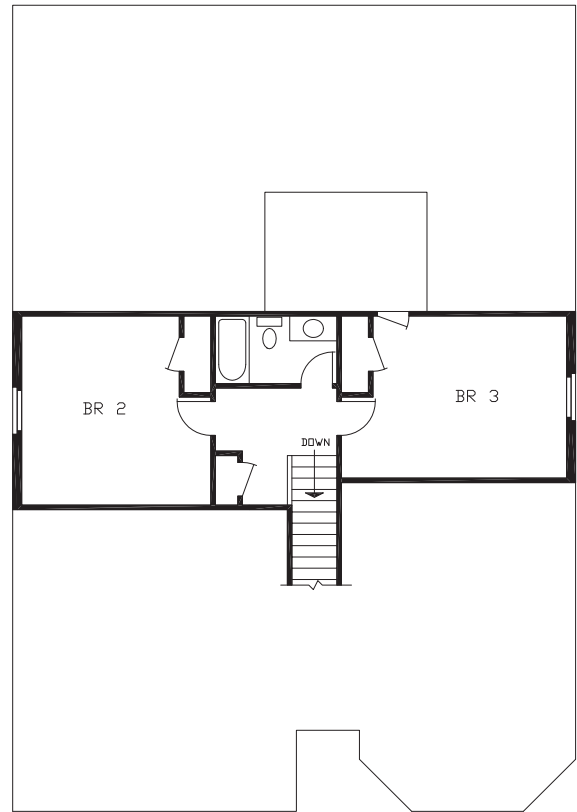
2ND FLOOR
